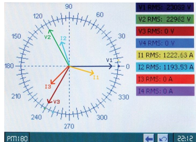
Phasor
